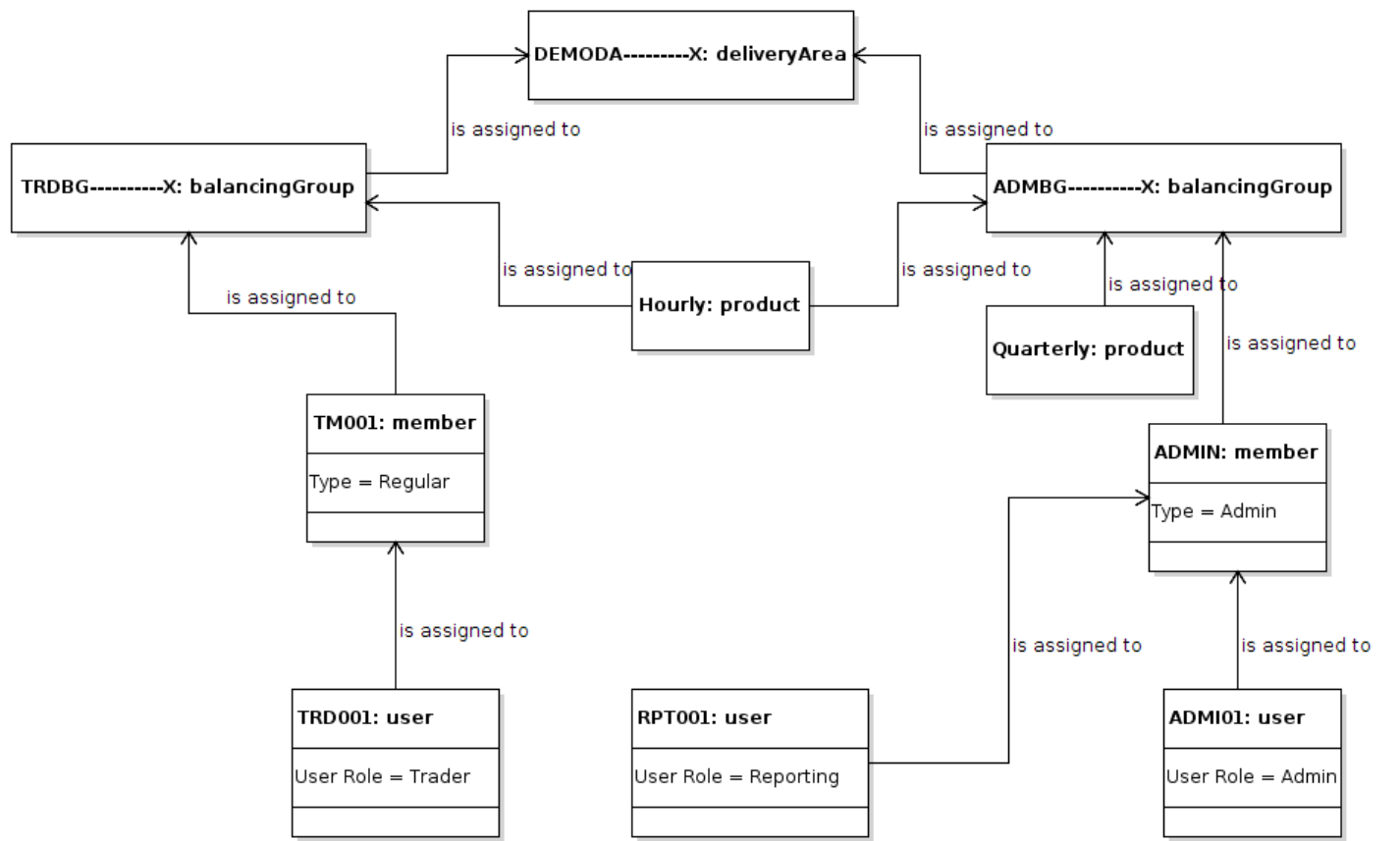
Figure 1: Instance Diagram
